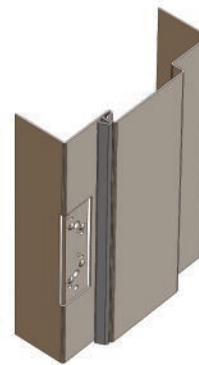
HINGE REINFORCEMENT
